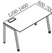
MONOFACE
